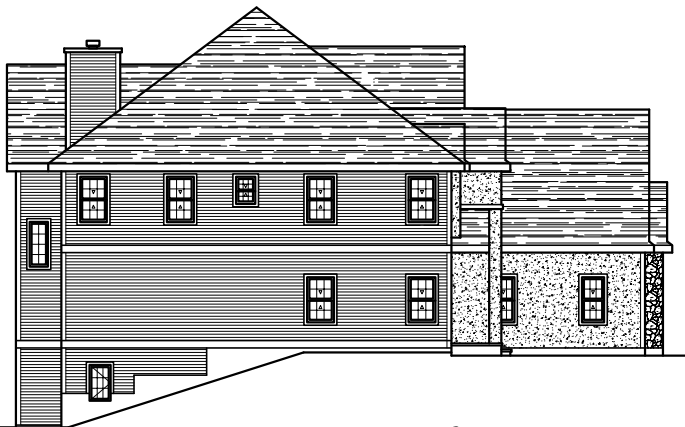
LEFT ELEVATION
