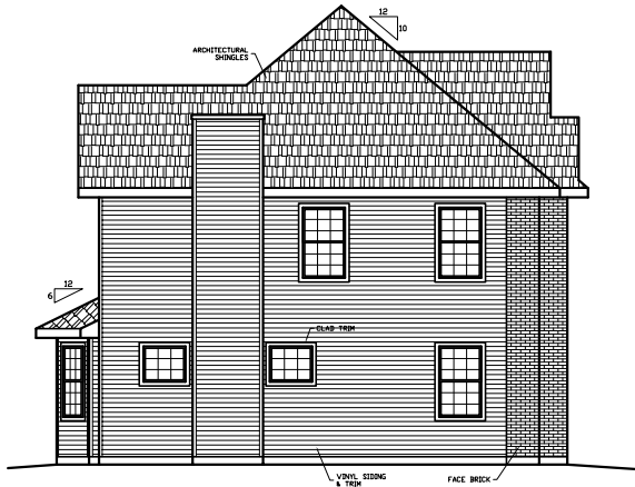
LEFT ELEVATION
