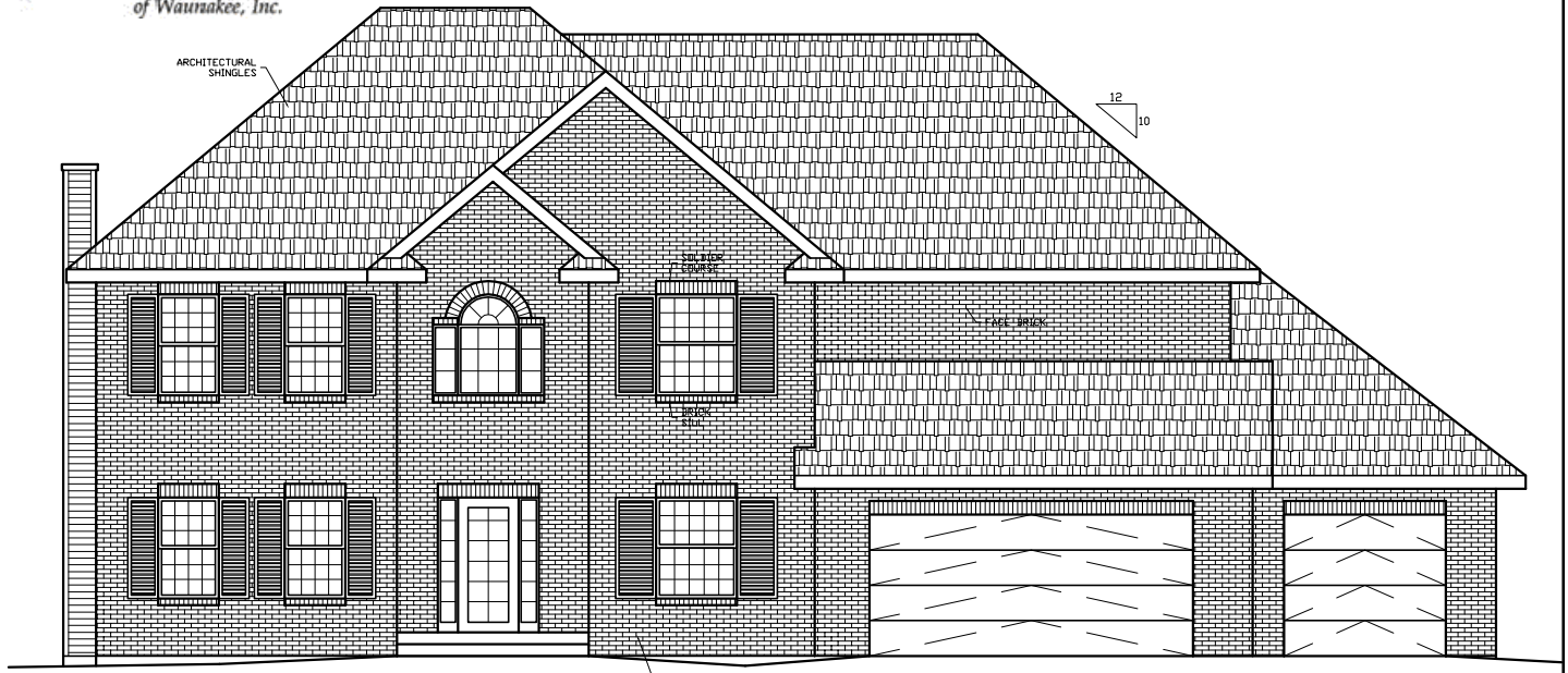
FRONT ELEVATION
