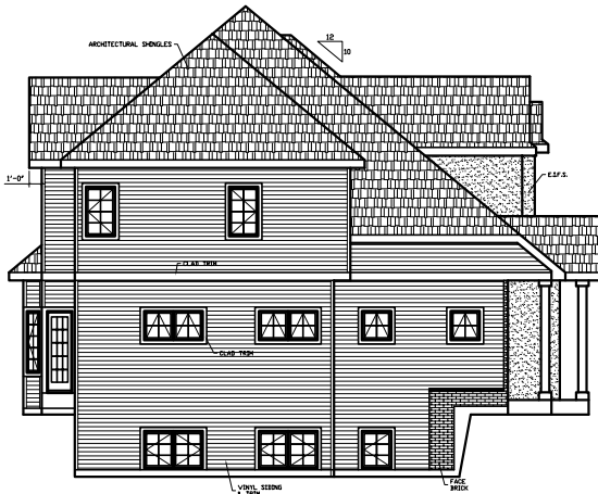
LEFT ELEVATION
