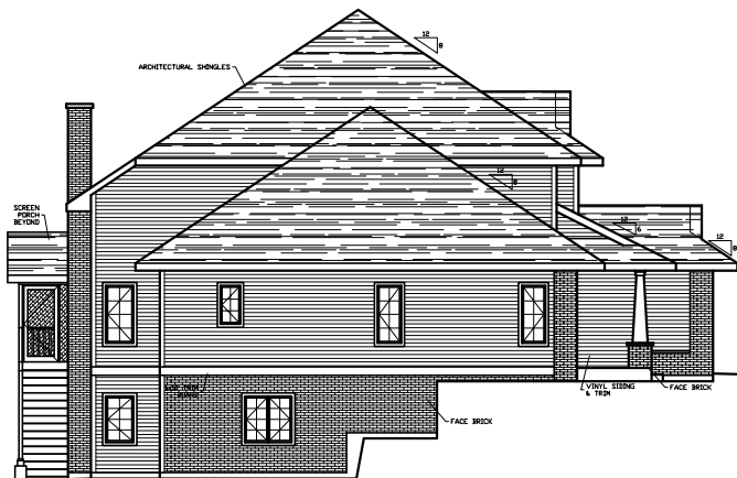
LEFT ELEVATION
