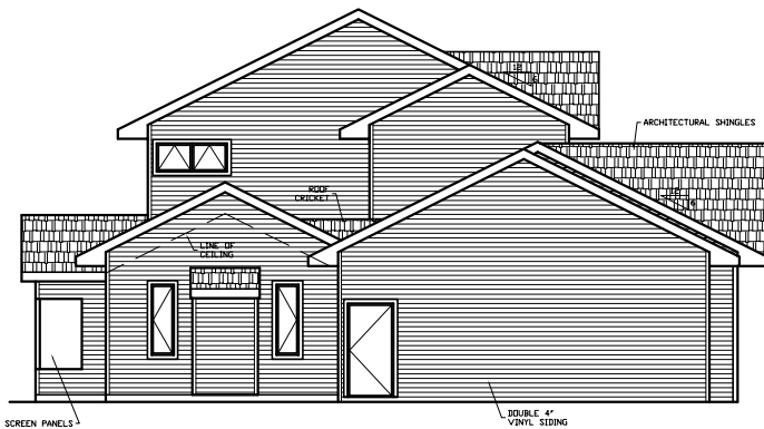
LEFT ELEVATION
