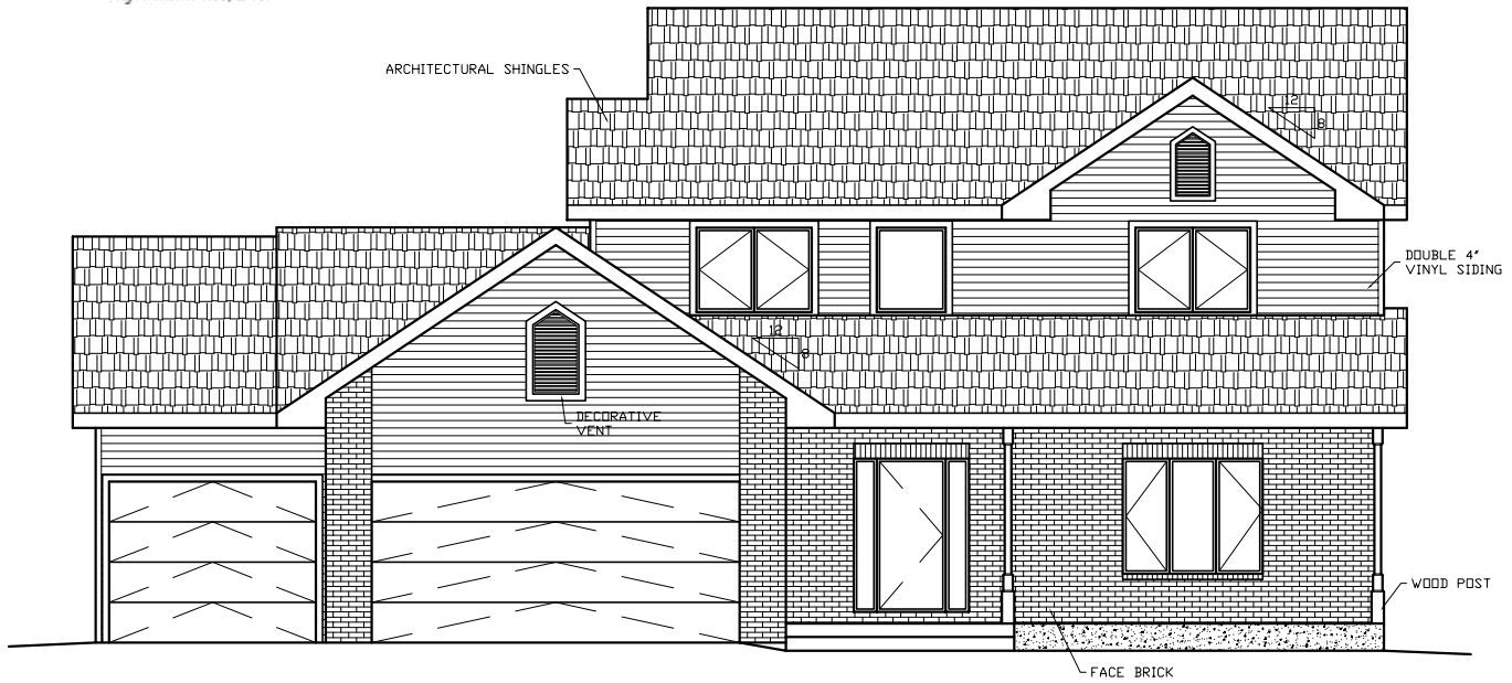
FRONT ELEVATION
