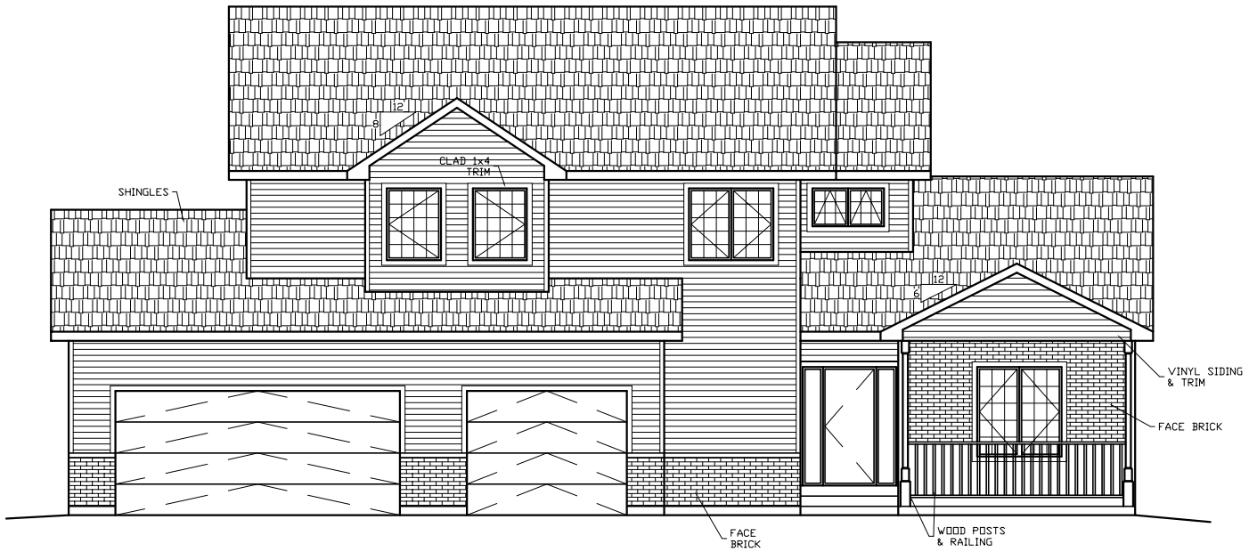
FRONT ELEVATION
