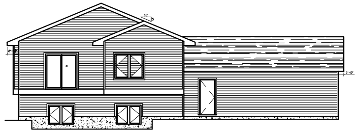
REAR ELEVATION
