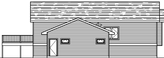
LEFT ELEVATION
