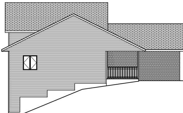
LEFT ELEVATION
