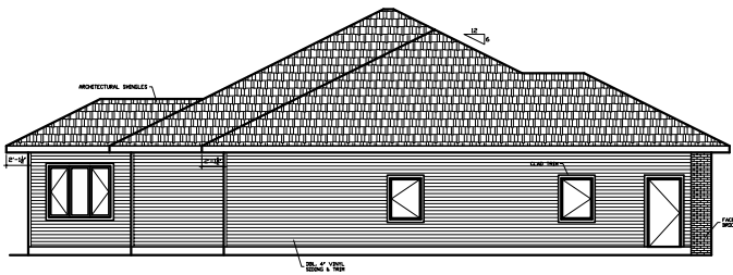
LEFT ELEVATION
