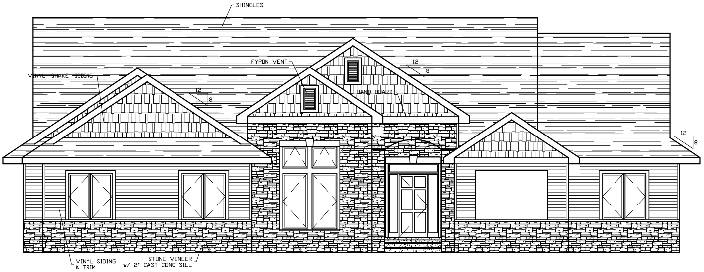
FRONT ELEVATION
