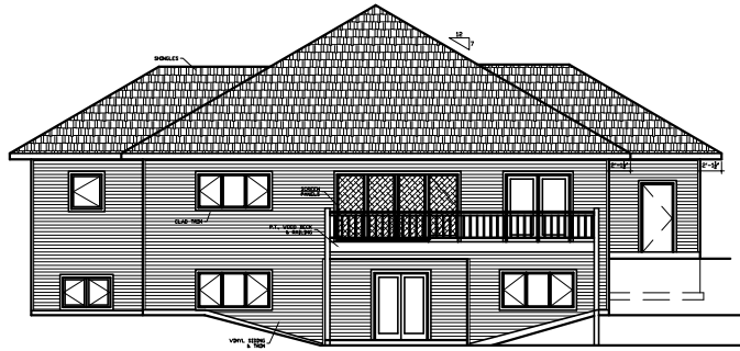
REAR ELEVATION
