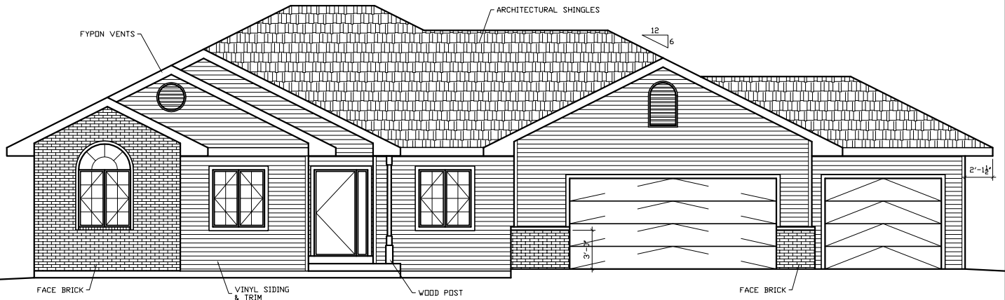
FRONT ELEVATION
