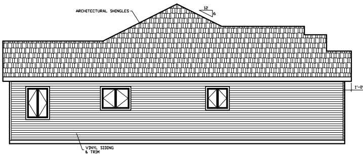
LEFT ELEVATION
