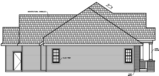
LEFT ELEVATION
