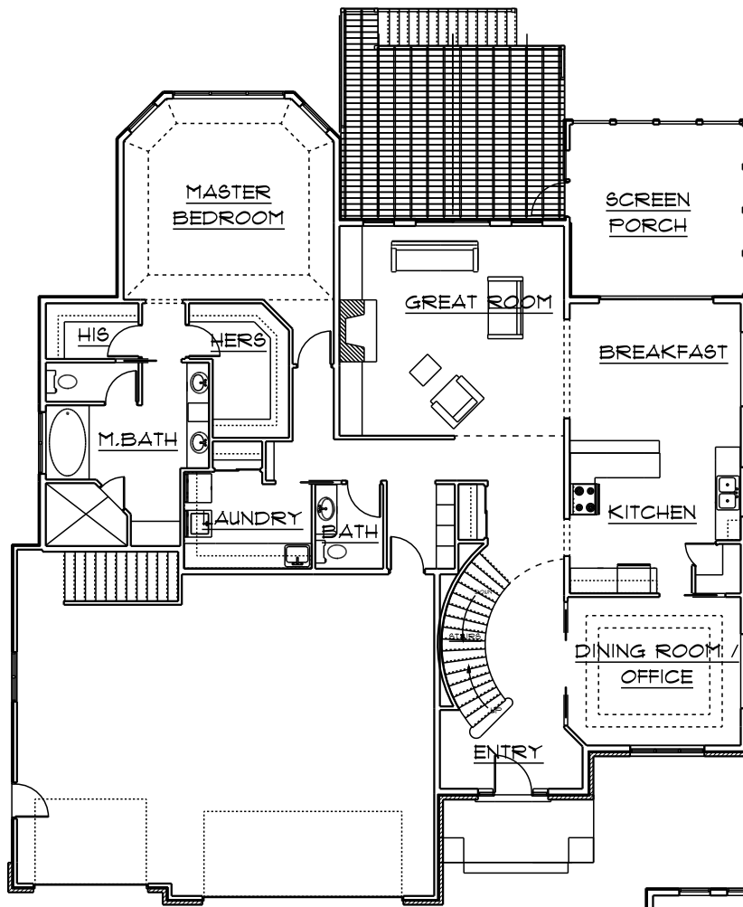
MAIN LEVEL
