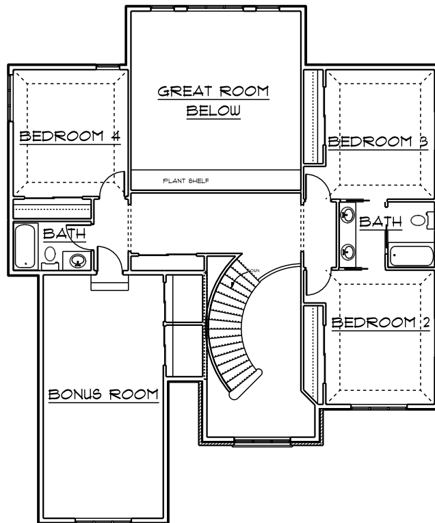
UPPER LEVEL
